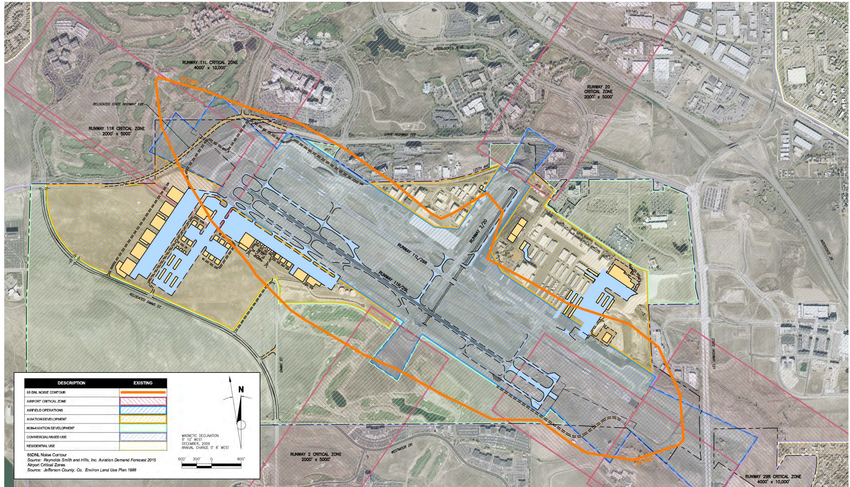
Figure 1-6 ON-AIRPORT LAND USE PLAN
